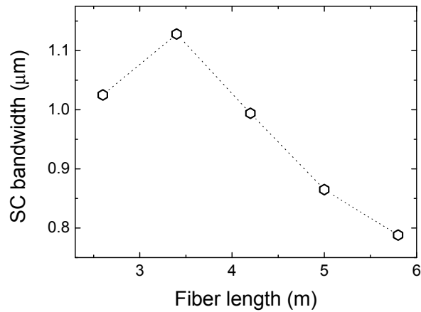
Fig. 7. Supercontinuum bandwidth (10 dB) as a function of \text{GeO}_2 fiber length.
