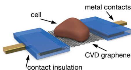
Fig. 114 Schematic GFET with a cardiomyocyte cell (a cell of muscular tissue in the heart) on the gate area. The metal contacts (in brown) are insulated from the electrolyte by two layers of chemically stable and biocompatible SU8 photoresist (blue rectangles). [Adapted from ref. 568].
