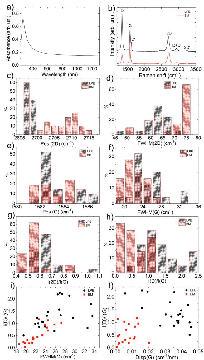
Figure 1. (a) Optical absorption of LPE dispersion diluted 1:12 with pure water/SDC. (b) Raman spectrum at 514.5 nm for representative LPE (black curve) and BM (red curve) flakes. Distribution of (c) Pos(2D), (d) FWHM(2D), (e) Pos(G), (f) FWHM(G), (g) I(2D)/I(G) , (h) I(D)/I(G) , and distribution of I(2D)/I(G) as a function of (i) FWHM(G) and (l) Disp(G) for LPE (black dashed histograms and dots) and BM (red dashed histograms and dots) flakes, respectively.
