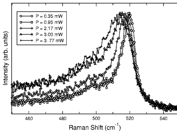
FIG. 1. Raman spectra of Si nanowires as a function of excitation power, see legend. The spectra were measured in air at a pressure p=0.1 mbar.
