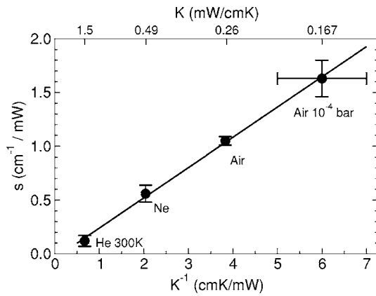
FIG. 4. Slope s of the SiNW frequency shift with excitation power vs inverse of the thermal conductivity K^{-1} of He, Ne, and air at 300 K (see labels). Thermal conductivities were taken from Ref. 19. Error bars are standard deviations when determining s from a linear regression.
