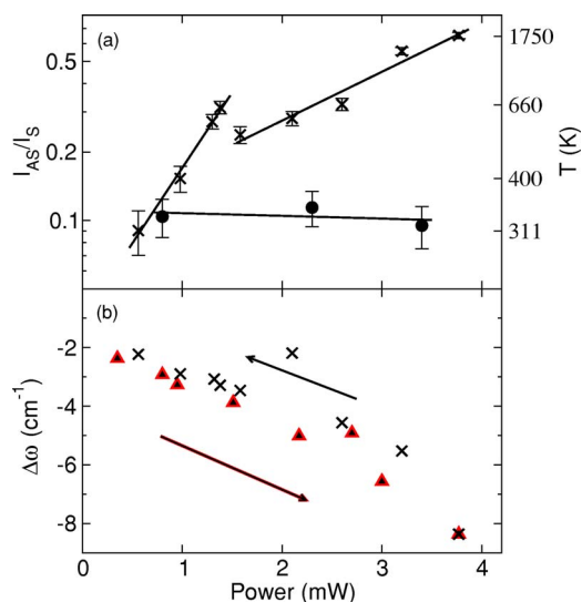
FIG. 2. (Color online) (a) Anti-Stokes/Stokes ratio of SiNWs (crosses) and bulk Si (circles). (b) Shift of the phonon frequency with respect to bulk silicon. Triangles (crosses) are peak positions for increasing (decreasing) laser power, see also arrows. The spectra were measured in air ( p=0.1 mbar).
