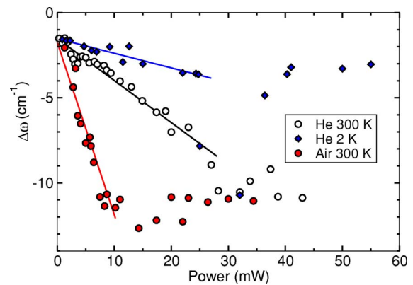
FIG. 3. (Color online) Phonon frequencies of SiNWs as a function of excitation power in He gas, air, and superfluid He. The lines are fits in the power ranges of linear frequency shift.
