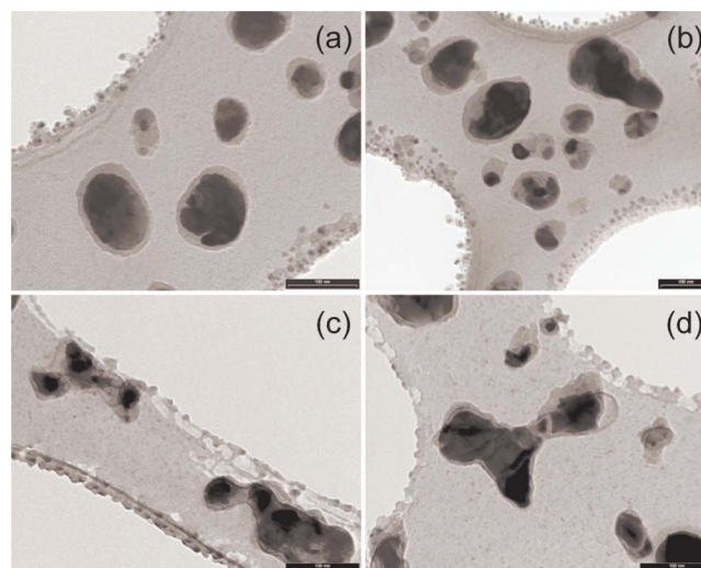
FIG. 9. (Color online) TEM images of 2 nm Ni films evaporated onto SiO_x , e-beam transparent grids, exposed to 50: 200 SCCM C_2H_2:NH_3 (0.7 mbar) at 450 °C for 5 min subjected to different pretreatments. (a) and (b) are pretreated in 200 SCCM 0.6 mbar NH_3 at 650 °C for 15 min, with 5 min dwell time at the same temperature and gas atmosphere. Grids in (c) and (d) are in NH_3 (200 SCCM, 0.6 mbar) at 650 °C for 15 min and applying a NH_3 plasma (600–700 V, <15 W) for 5 min.
