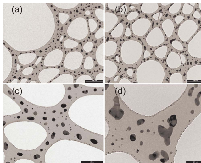
FIG. 8. (Color online) TEM images of 2 nm Ni films evaporated onto SiO_x , e-beam transparent grids, then subjected to different pretreatments. Grids in (a) and (c) are pretreated in NH_3 (200 SCCM, 0.6 mbar) at 650 °C for 15 min, followed by a 5 min dwell time at the same temperature and gas atmosphere. Grids in (b) and (d) are heated up in NH_3 (200 SCCM, 0.6 mbar) to 650 °C in 15 min and applying a NH_3 plasma (600–700 V, <15 W) for 5 min.
