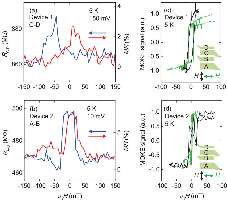
FIG. 2. MR and MOKE at 5 K. Resistance R(H) and magnetoresistance MR(H) = \Delta R(H)/R_{\min} measured between (a) electrodes C-D (device 1, bias 150 mV) and (b) A-B (device 2, bias 10 mV), with magnetic field H applied along electrode widths. (c) and (d) MOKE signal from nearby wirebond pad, with H applied along electrode widths (black data) and lengths (green data). Hard-axis data in (d) show an unexpected discontinuity. Resistance data are averaged over 3 [device 1] and 10 [device 2] sweeps of magnetic field. Raw data appear in supplementary note 5. 34
