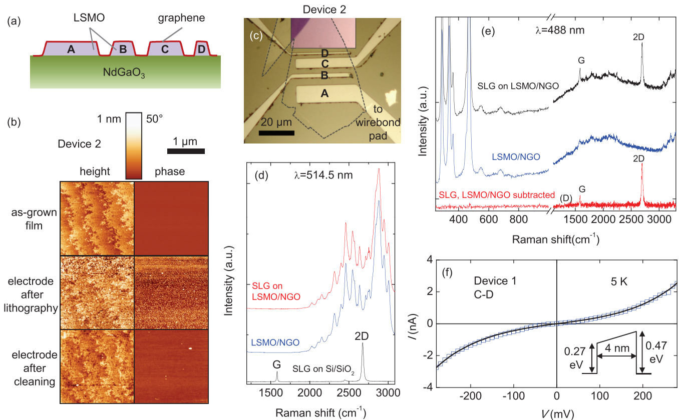
FIG. 1. Graphene and LSMO electrodes. (a) Device schematic showing LSMO electrodes A–D, conformally coated with SLG (red) [electrode widths are A (10 \mu\text{m} ), B (3 \mu\text{m} ), C (6 \mu\text{m} ), and D (2 \mu\text{m} )]. Electrode spacings are A-B (3 \mu\text{m} ), B-C (2 \mu\text{m} ), and C-D (1 \mu\text{m} ). (b) AFM images of an electrode in device 2 at different stages of processing. (c) Composite optical microscopy image, showing SLG (purple) on \text{SiO}_2 (pink) before transfer (rectangular region at top), and on LSMO electrodes in device 2 after transfer (rest of image). (d) Raman spectra of graphene on \text{SiO}_2 before transfer and on LSMO/NGO after transfer. (e) Raman spectra of graphene on LSMO/NGO after transfer showing background correction. (f) Current ( I ) versus voltage ( V ) for electrodes C and D of device 1 at 5 K (open symbols), and from a Brinkman fit for back-to-back asymmetric tunnel barriers (black line). Inset: fitted barrier shape.
