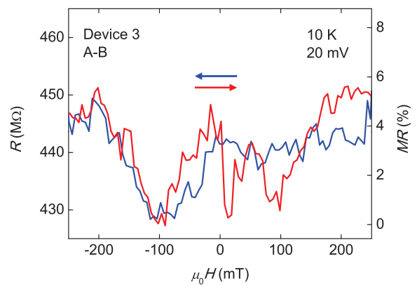
FIG. 3. MR at 10 K with out-of-plane applied field. Resistance R(H) and magnetoresistance MR(H) = \Delta R(H)/R_{\text{min}} measured between electrodes A-B (device 3, bias 20 mV), with magnetic field H applied out of the LSMO film plane. Resistance data are averaged over 10 sweeps of magnetic field. Raw data appear in supplementary note 5. 34
