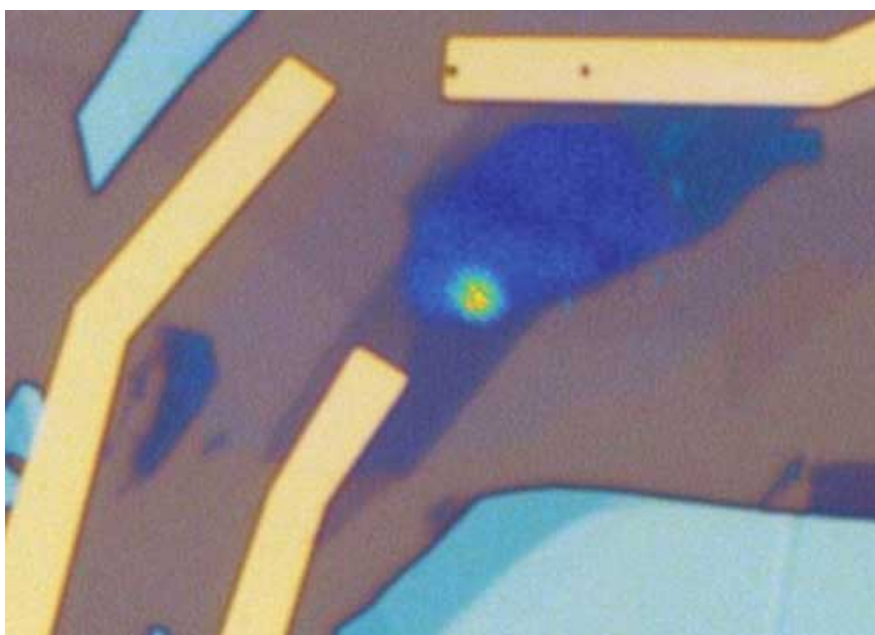
An overlay of the microscope image of a quantum LED device and the photoluminescence image from the active area of WSe 2 . The isolated bright spot corresponds to a quantum emitter generating a stream of single photons. (Image: Mete Atatüre)
