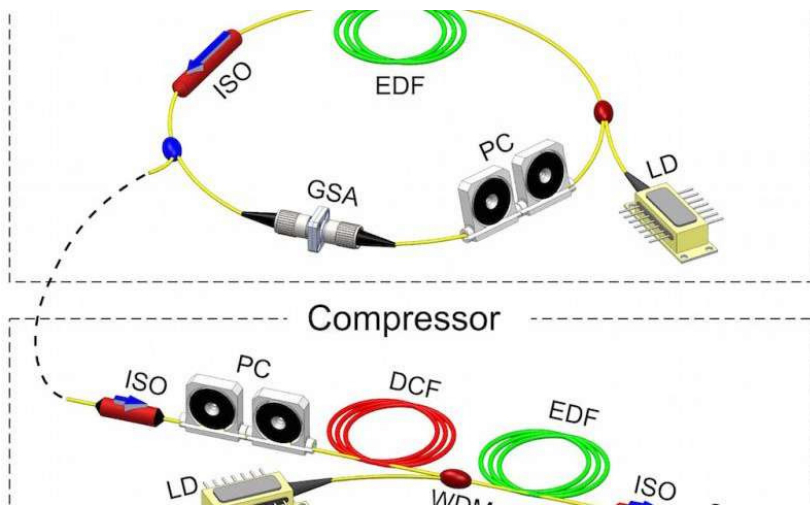
Schematic of an all-fibre laser capable of producing few-cycle pulses. Laser pulses of length 263 femtoseconds are produced from a seed oscillator (top) mode-locked using a graphene-based saturable absorber. These pulses are fed through a ... more
